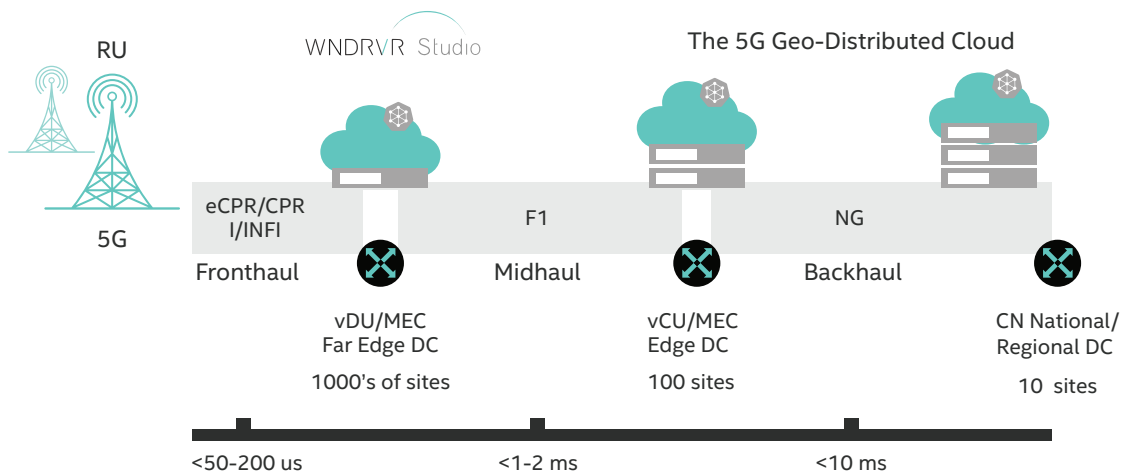
Figure 1. Wind River Studio Cloud Platform deployed as a single geo-distributed cloud.
