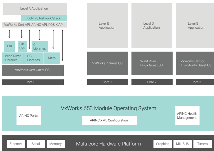
図 2. IMA design with VxWorks 653 Multi-core Edition
